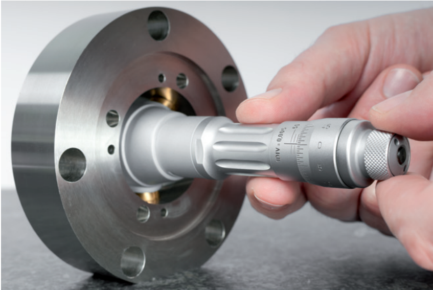
Bore measurement with a BROWN & SHARPE INTRIMIK inside micrometer
