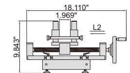
adaptor (optional, for digital torque tester IST-TT5, IST-TT50, IST-TT220)
