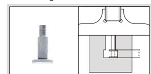
1148-P103E (optional), measure width of bottom grooves inside blind hole
