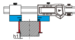
Measuring external groove diameter with flat measuring face (depth h1 \leq 0.098" )
