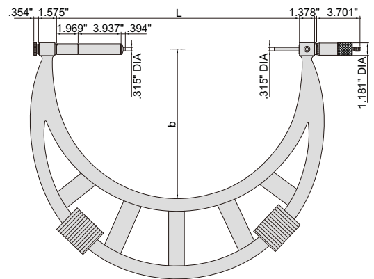
adjust collars for different measuring ranges
