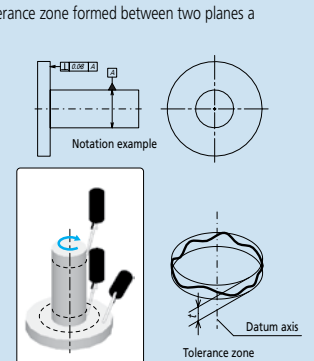
Verification example using a roundness measuring instrument
